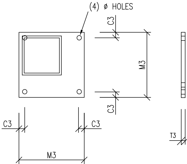
CORNER BASE PLATE
