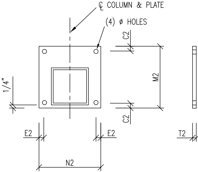
OFFSET BASE PLATE
